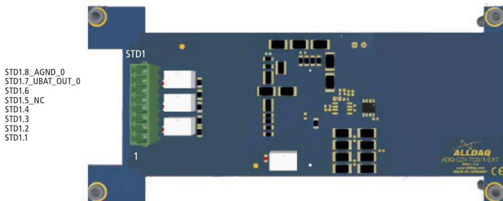
Figure: ADQ-CDI-TCU/1 EXT4 including pin assignment
